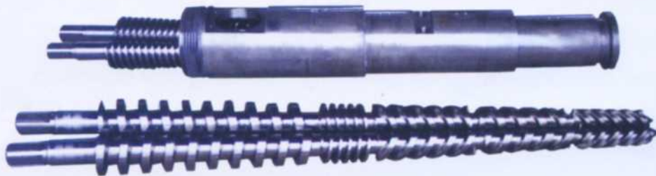
Conical Twin Screw & Barrel
